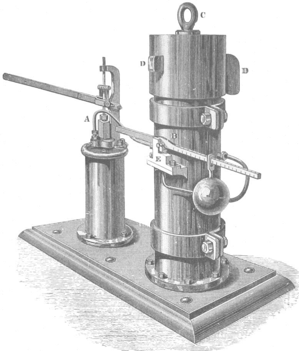
FIG. 13.—The Hydraulic Pump.
